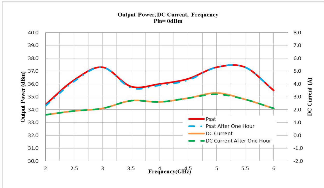
Graph1: Output Power (Low temp. -20±3°C)
