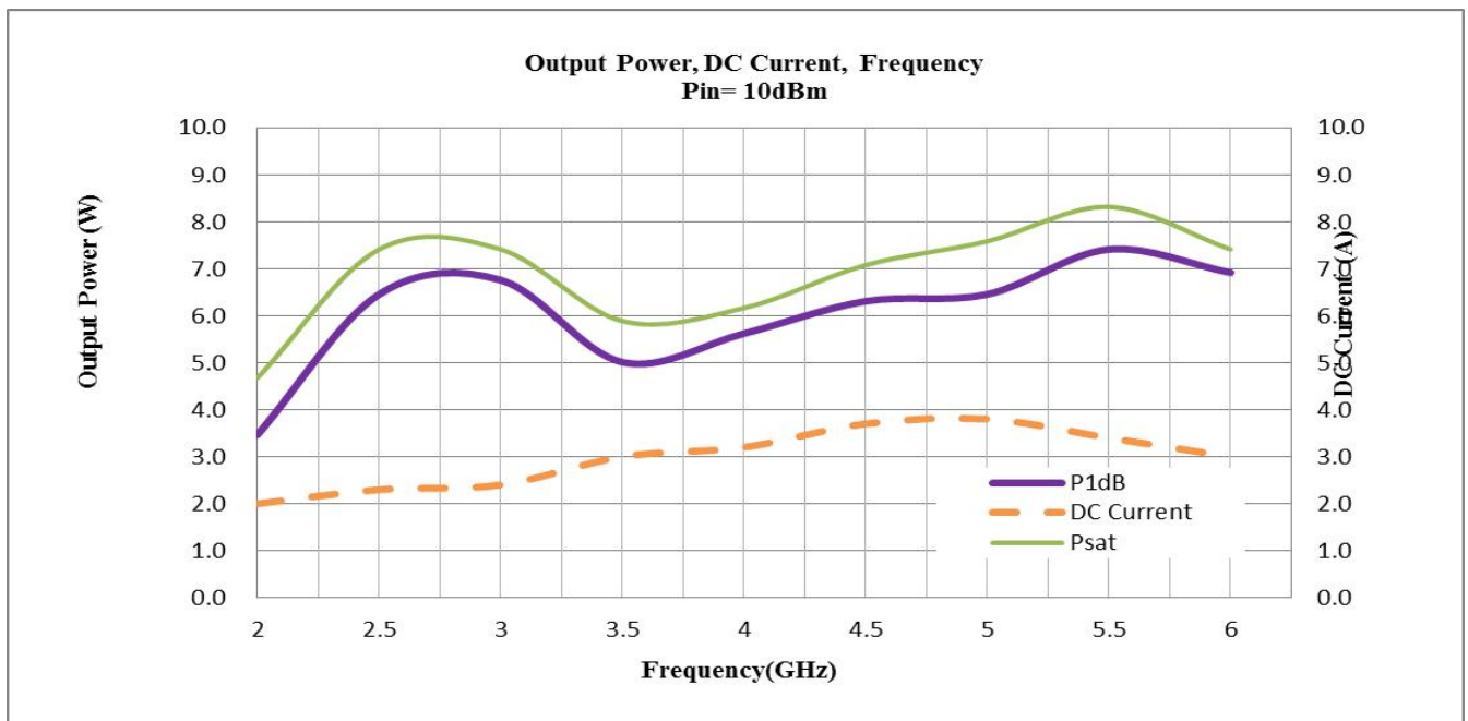
Graph3: Output Power (Normal temp. +25±3°C)
